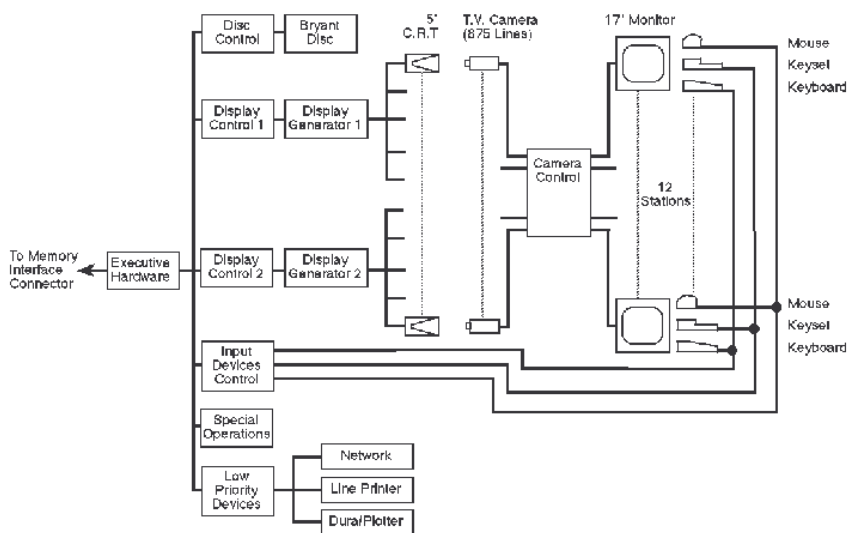
Figure 10--Special devices channel
