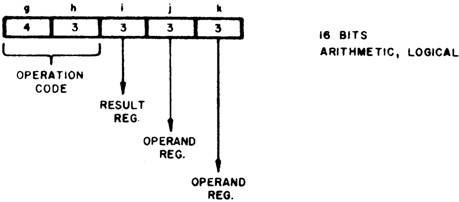
Figure 4-2. Format for arithmetic and logical instructions
